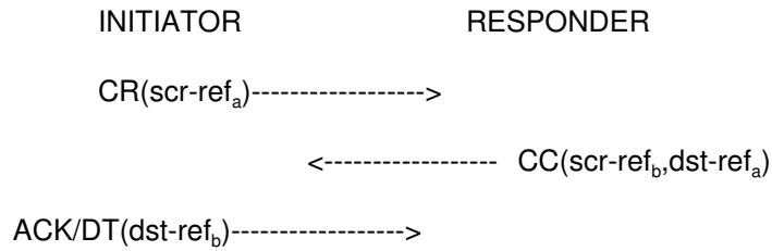
Figure 3: Illustration of exchanges to support peer entity authentication.
